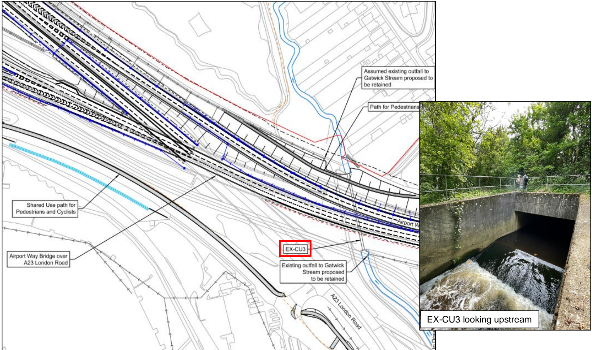
Figure A. 4: Proposed Drainage Strategy Drawing, indicating EX-CU3, and associated photos
